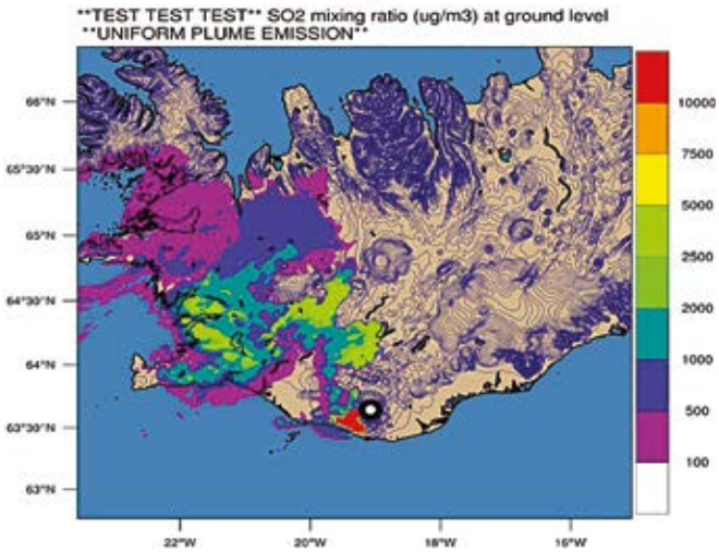
Figure 1. Weather Research and Forecasting (WRF) model simulation of the concentration of sulphur dioxide in Iceland, 42 hours after the start of the eruption. The location of the eruption, Katla, is marked with a white circle. Note the complex pattern of gas dispersion, associated with the topography of Iceland and the prevailing meteorological conditions.
